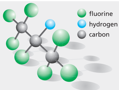
HFC-227ea molecule
